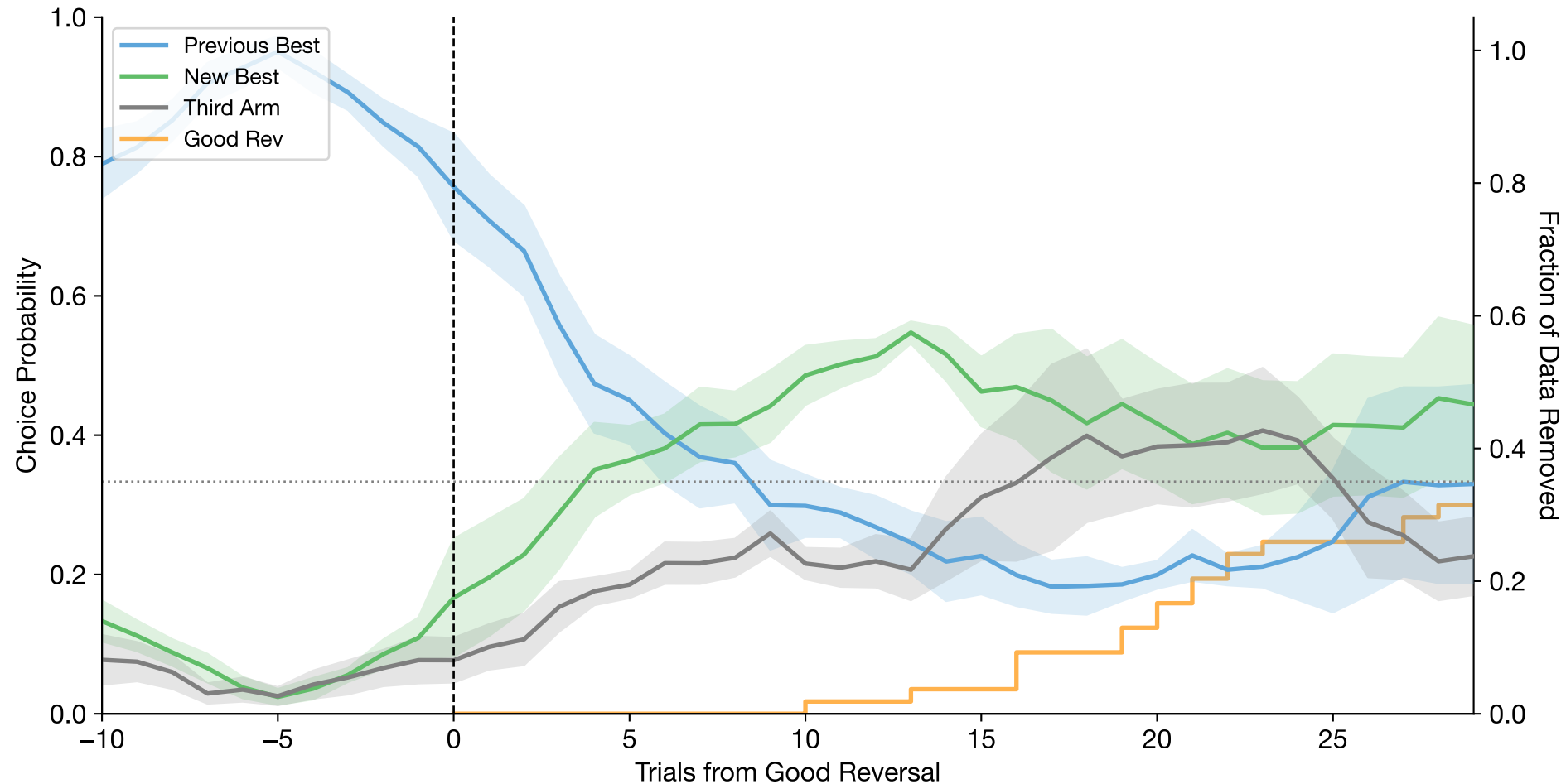
Good Reversal-Aligned Choices (mean \pm se across subjects | n=6 subjects, n=54 reversals)
